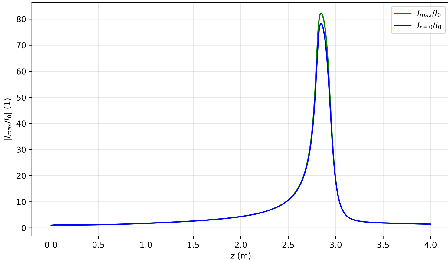
I_{max}(x = 0, y = 0, z)/I_0 , P_{in}=1.2P_{cr} , noisy input, artificial time
